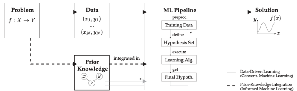
Figure 1. The information flow in gTransformer, following the taxonomy proposed by Von Rueden et al. [17], comprises: (1) Prior Knowledge : simulation results from an educational model serve as a source of structured information; (2) Training Data : the augmented data is used to train the model; (3) Hypothesis Set : an attention-based Transformer architecture provides the inductive bias required to align internal representations with the reference model; (4) Learning Algorithm : optimization is driven by a compound loss function, which guides the system toward semantically aligned representations; and (5) Final Hypothesis : the internal representations are projected and compared with the prior knowledge of the reference model.
