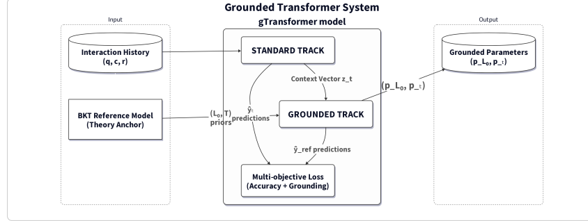
Fig. 1: The gTransformer architecture. The model integrates theoretical priors and interaction history to produce student-specific grounded parameters through parallel standard and grounded tracks.
