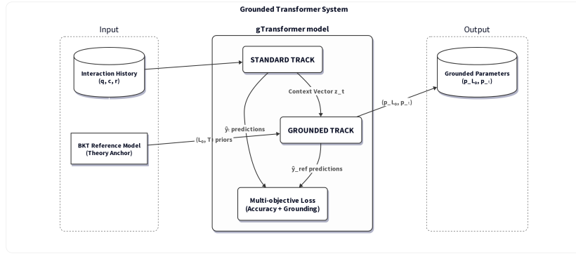
Fig. 1: The gTransformer architecture. The model integrates theoretical priors and interaction history to produce student-specific grounded parameters through parallel standard and grounded tracks.
