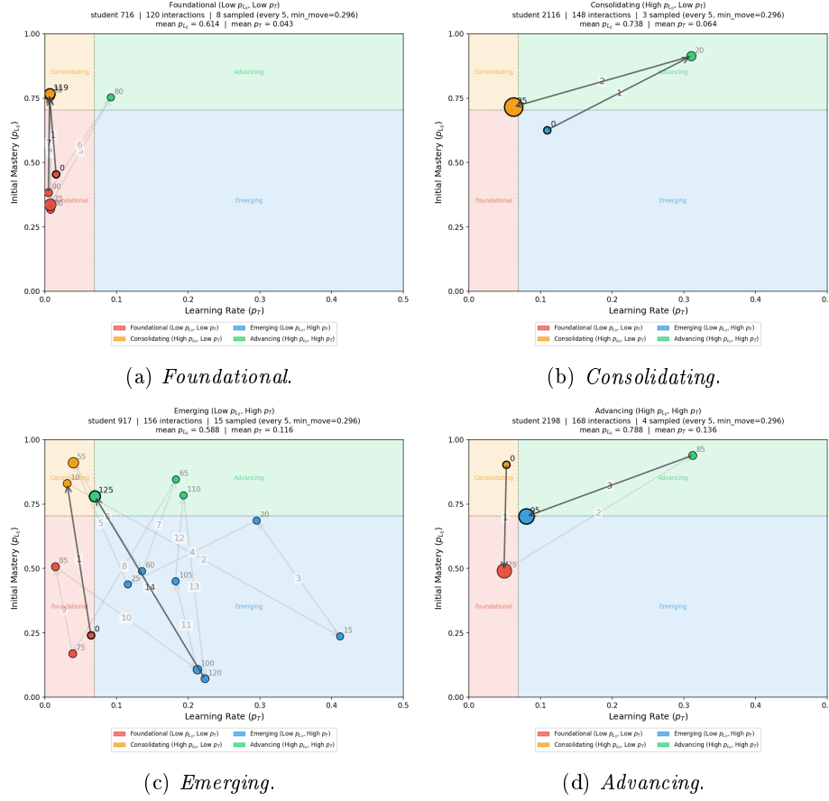
Fig. 4: Learning situation trajectories. Movement of the grounded parameters pair (p_T, p_{L_0}) over time. Marker area encodes dwell time.
