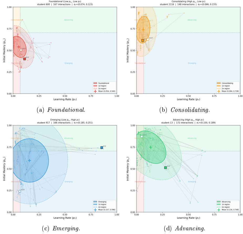
Fig 3: Parameter orbit ellipses. Covariance ellipses (1-sigma and 2-sigma) for the representative student of each quadrant ( p_{L0} , p_T ).
