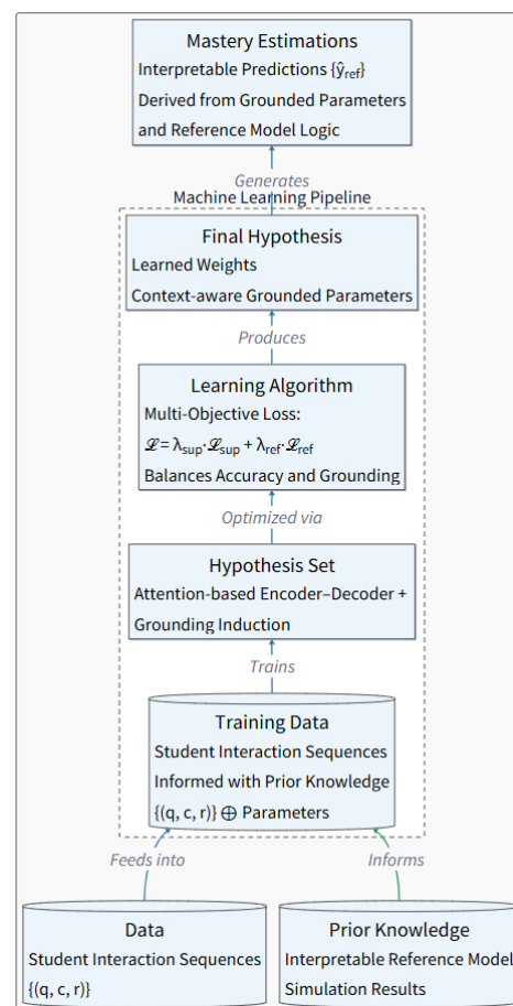
Figure 1. Dimensions of Informed Machine Learning (IML) in gTransformer.
