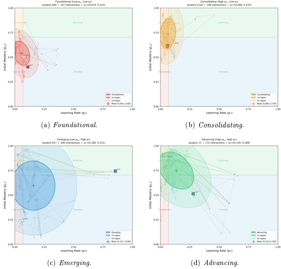
Fig. 2: Parameter orbit ellipses. Covariance ellipses (1-sigma and 2-sigma) for the representative student of each quadrant ( p_L , p_T ).
