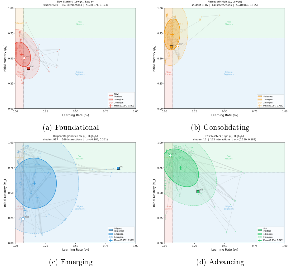
Fig 3: Parameter orbit ellipses. Covariance ellipses ( 1\sigma and 2\sigma ) for the representative student of each learning situation in (p_{L_0}, p_T) space. The centre marks the mean parameter position; ellipse shape encodes the extent and orientation of parameter variability across all interactions.
