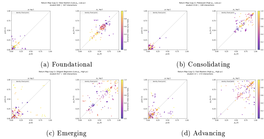
Fig. 4: Return maps. Lag plots for the representative student of each learning situation. Each panel shows p_{L_0}(t+1) vs p_{L_0}(t) (left) and p_T(t+1) vs p_T(t) (right). Points are coloured from dark (early) to bright (late) interactions. The diagonal (dashed line) marks the fixed point; deviations above indicate increasing parameters and deviations below indicate decreasing ones.
