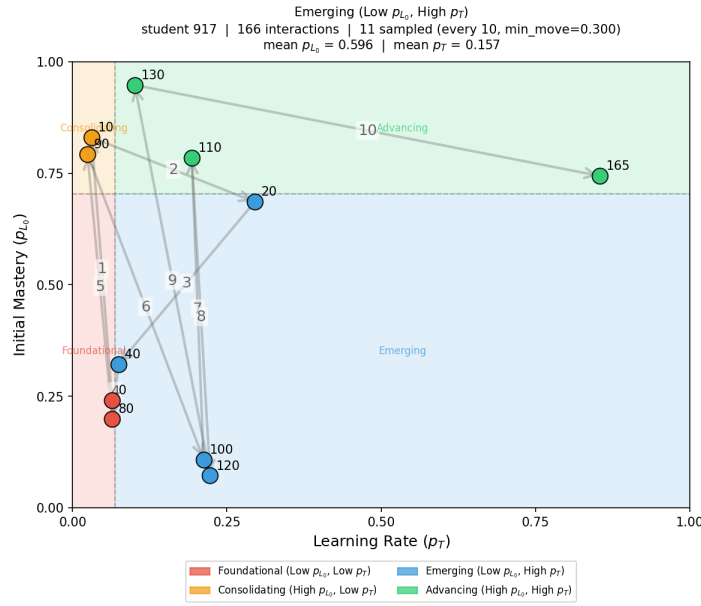
(a) Emerging (low p_{L_0} , high p_T ): spatially extended trajectory crossing quadrant boundaries; high learning rate signals strong growth potential.
