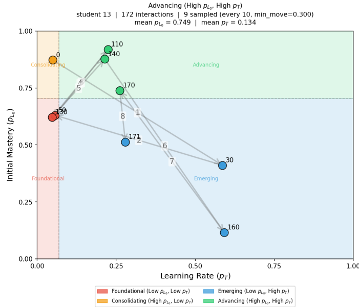
(b) Advancing (high p_{L_0} , high p_T ): upper-right trajectory with moderate spread; robust mastery across contexts supports routing to accelerated content.
