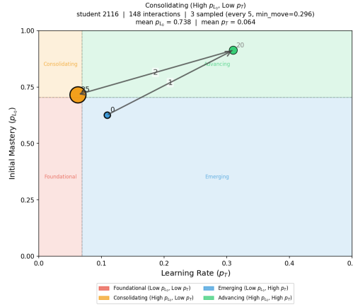
(b) Consolidating (high p_{L0} , low p_T ).
