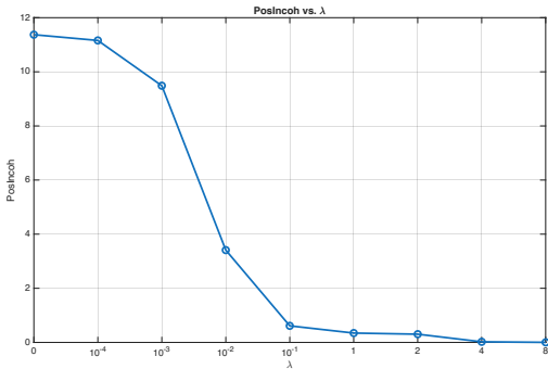
Fig. 6: Effect of \lambda on basis diversity and reconstruction (on zoo dataset, other datasets follow similarly). Increasing \lambda reduces positive basis correlations, as measured by \text{PosIncoh}(\mathbf{F}) .
