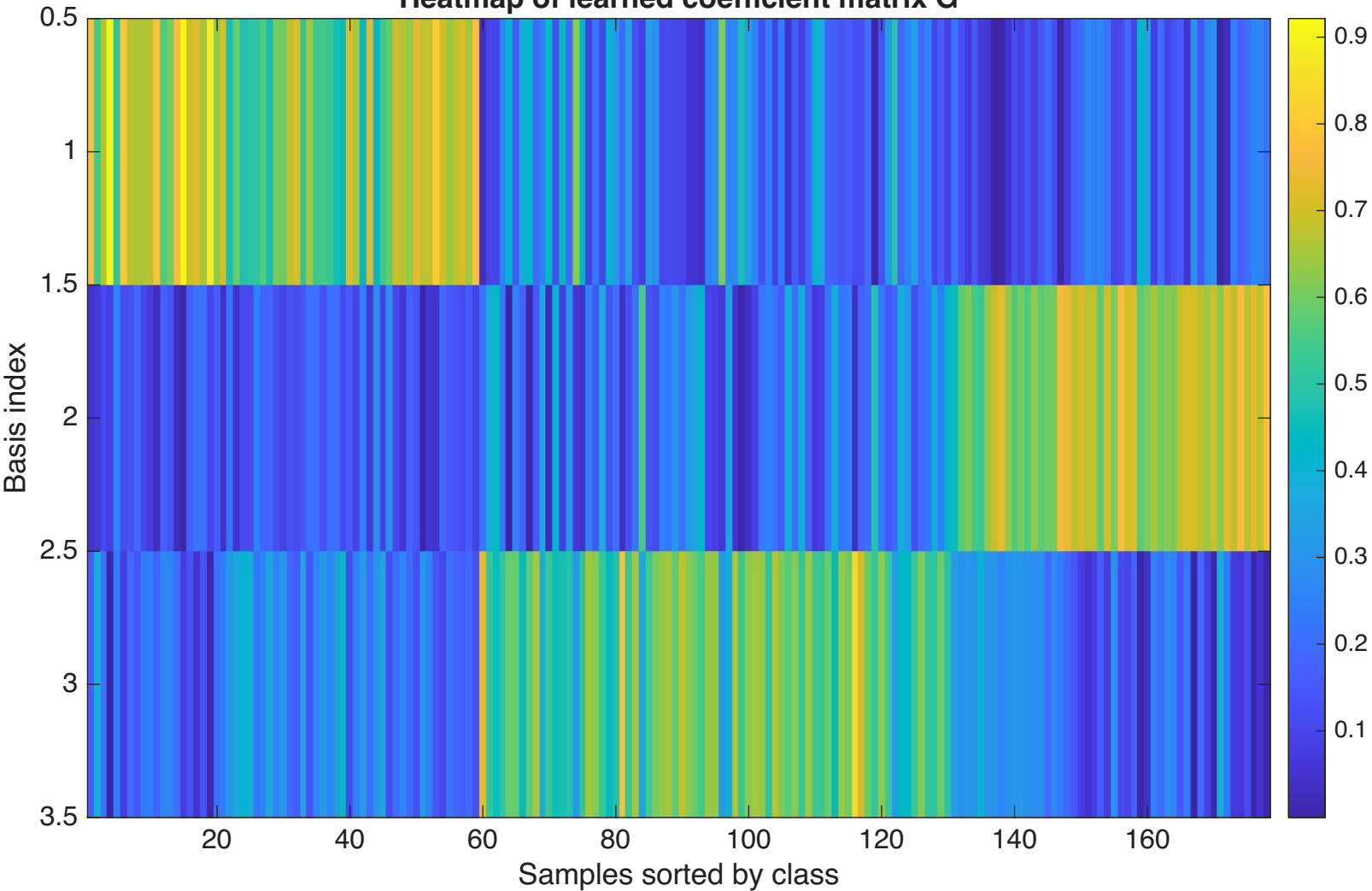
Heatmap of learned coefficient matrix G
