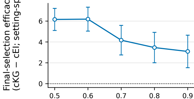
(c) MARIPOSA-motivated
