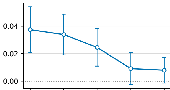
(b) Logistic
