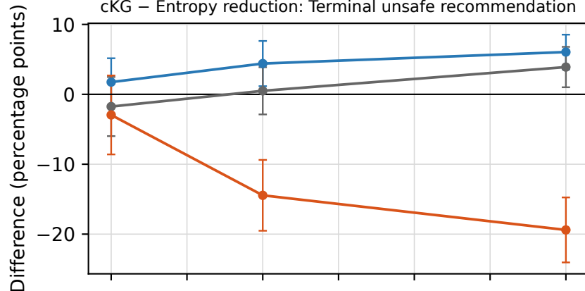
cKG – Entropy reduction: Terminal unsafe recommendation
