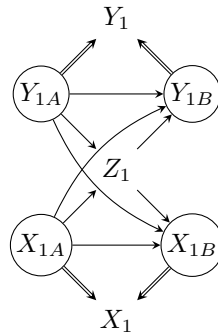
Figure 1: Reciprocity due to composite period variable. Circled variables are latent. Double-arrows indicate observed variables are composite variables determined by their parents
