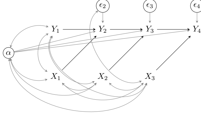
Figure 5: Maximum likelihood structural equation fixed-effects dynamic panel model with only lagged effects, adapted from Allison et al. (2017)
