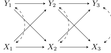
Figure 4: A theoretical model of cross-lagged effects with ambiguous contemporaneous relations.
