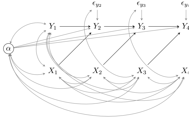
Figure 5: Maximum likelihood structural equation fixed-effects dynamic panel model (Allison et al., 2017)
