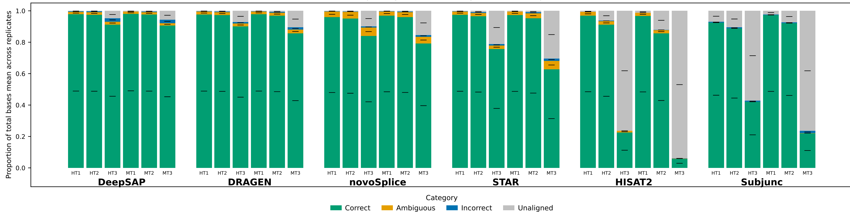
Baruzzo base-level metrics per aligner (95 % CI range; 500 bootstraps × 20000000 reads)
