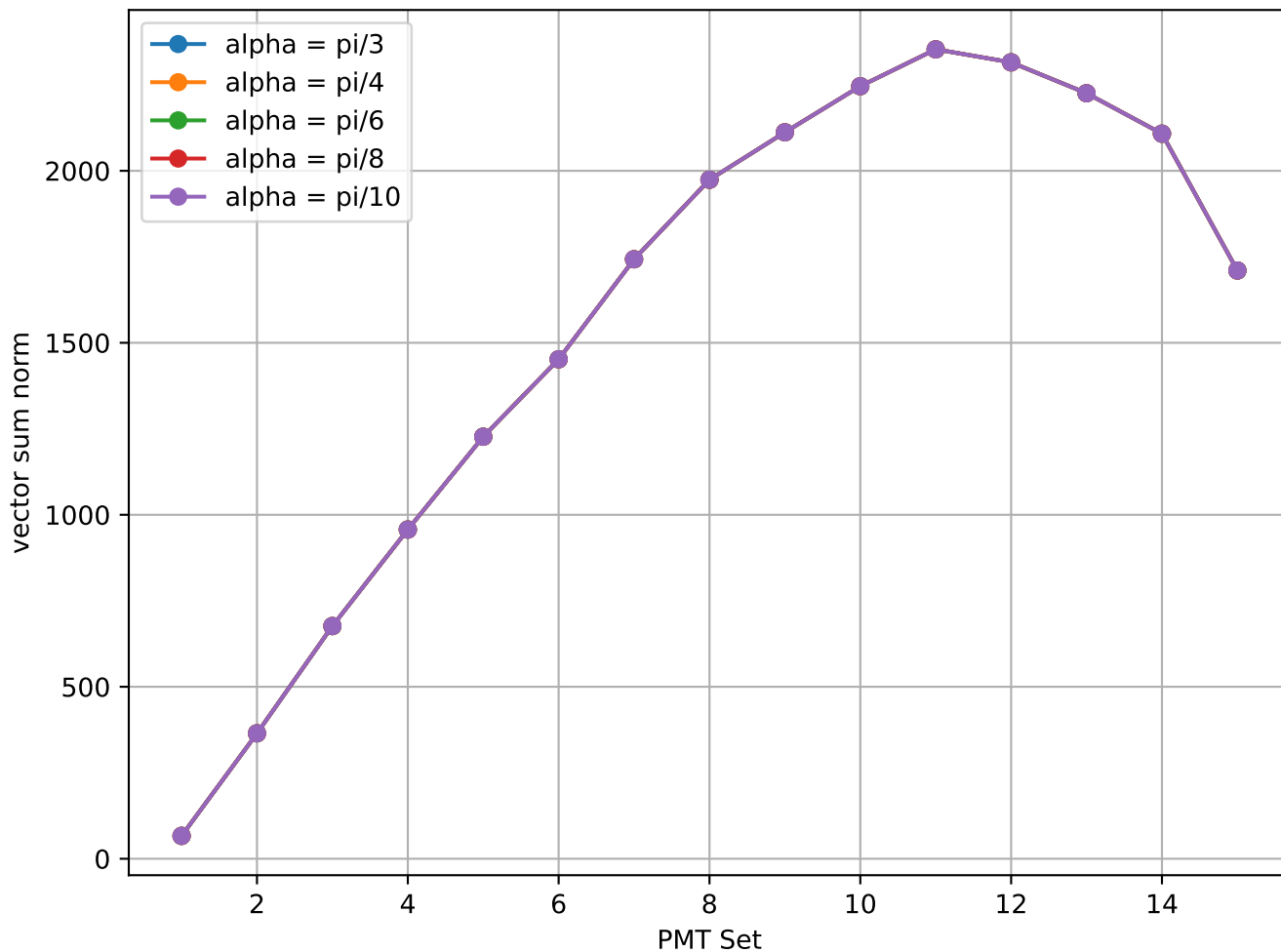
vector sum norm vs PMT Set
