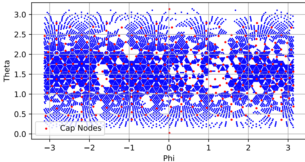
PMTs map for run 364600
