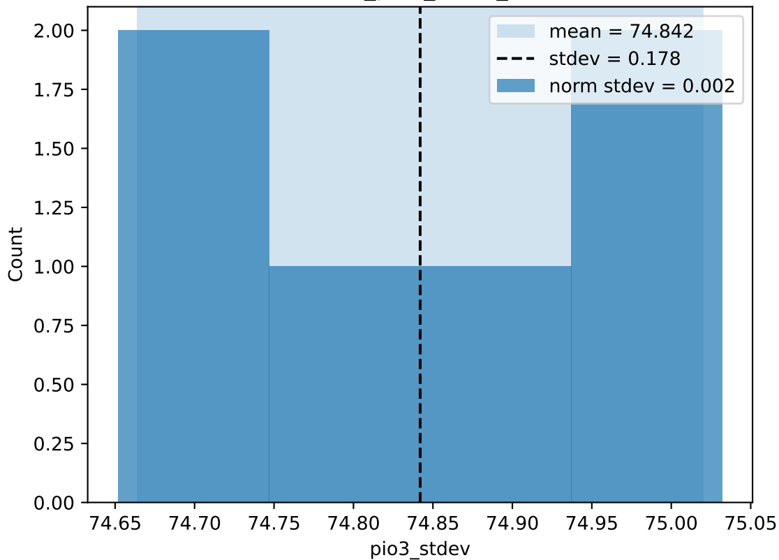
random_pio3_stdev_stats
