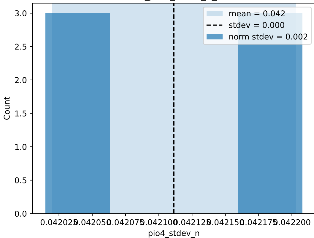
random_pio4_stdev_n_stats
