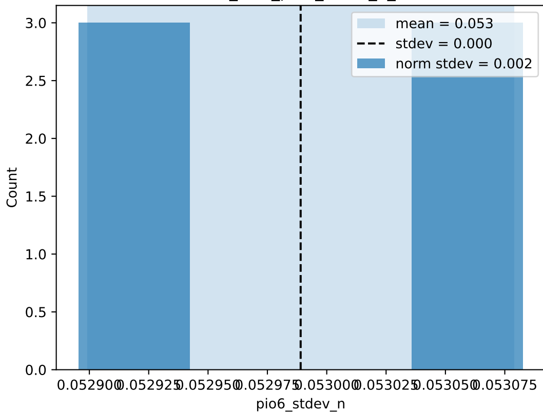
random_new_pio6_stdev_n_stats
