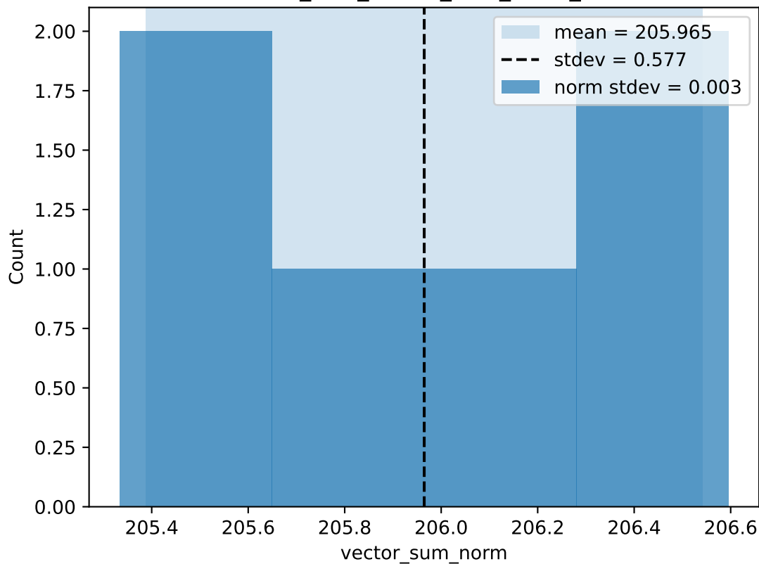
random_new_vector_sum_norm_stats
