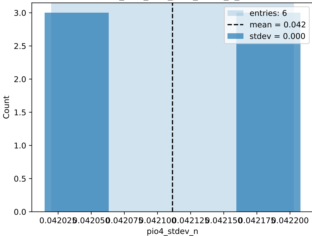
random_new_new_pio4_stdev_n_stats
