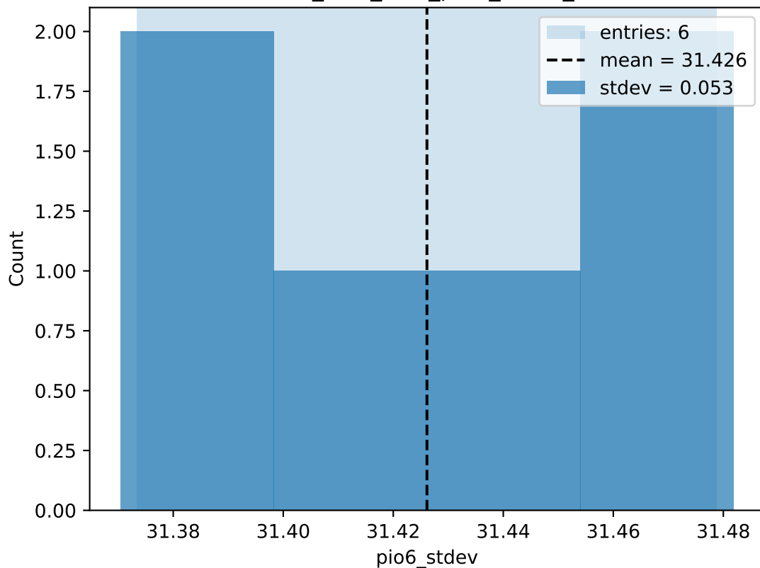
random_new_new_pio6_stdev_stats
