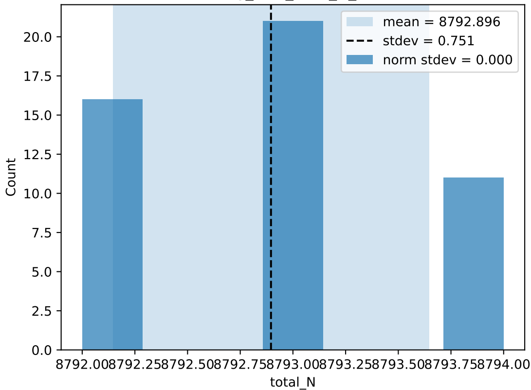
testing_new_total_N_stats
