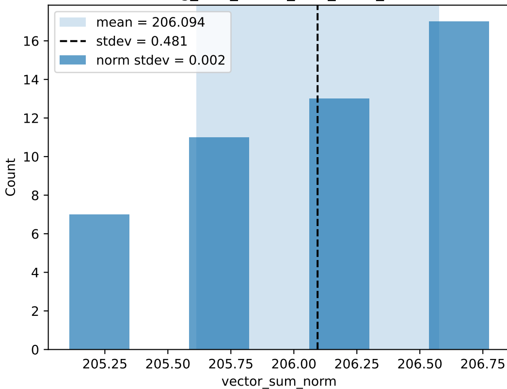
testing_new_vector_sum_norm_stats
