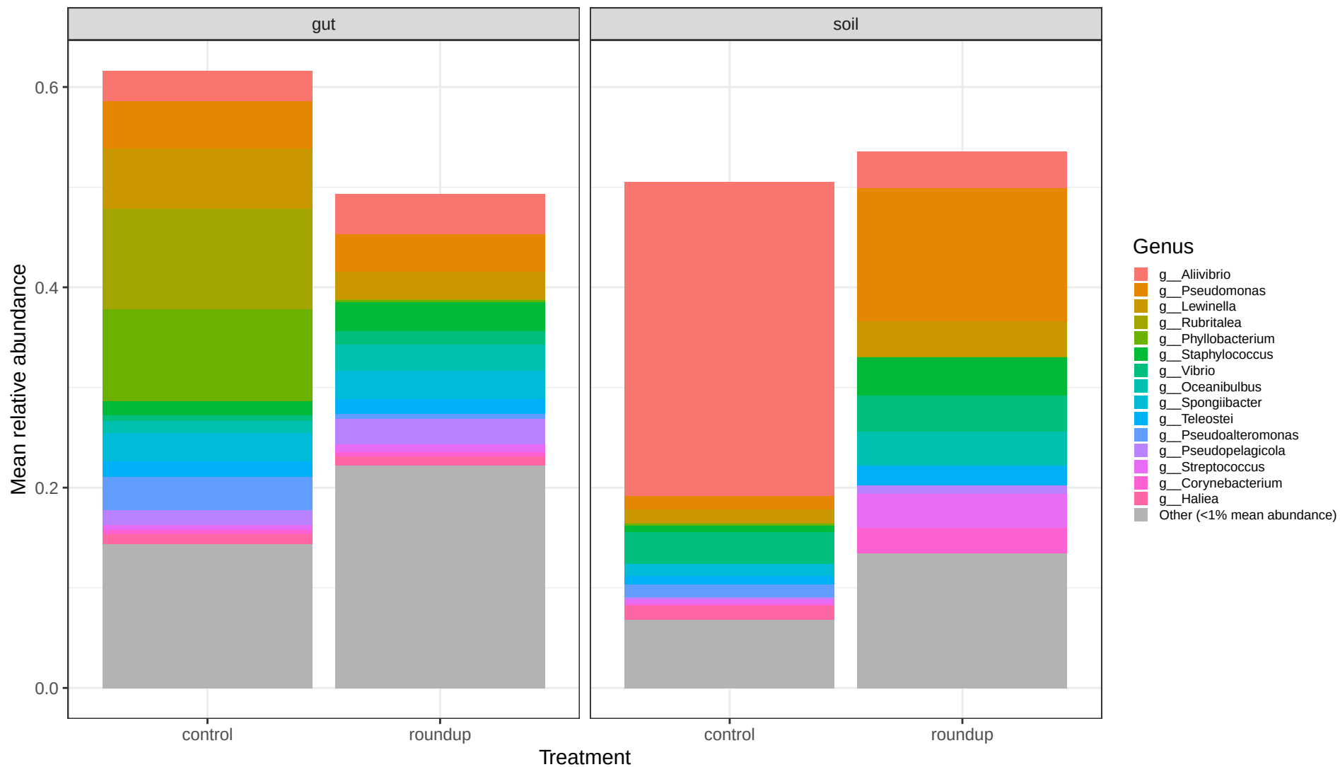
Treatment-averaged taxonomic composition (genus level)
