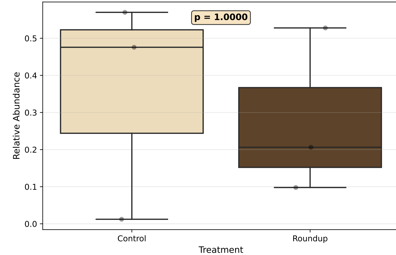
Class II (Resistant) by Treatment Soil Compartment
