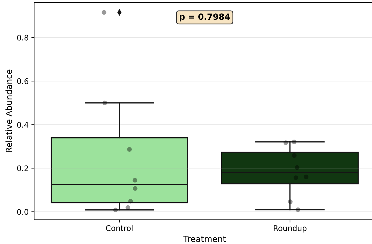
Class II (Resistant) by Treatment Gut Compartment
