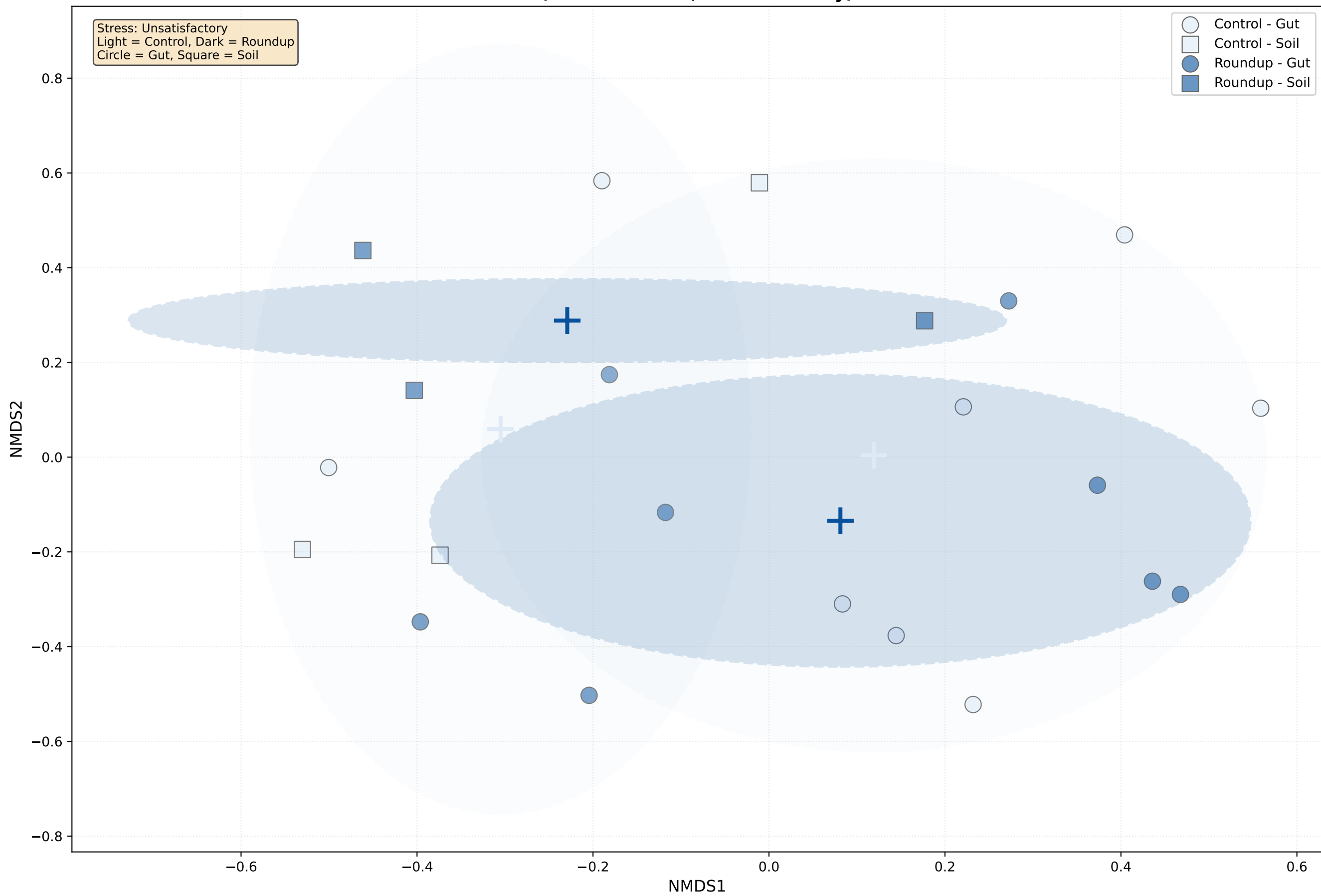
NMDS Ordination (3D) - Bray-Curtis Distances (Stress = 0.414, Unsatisfactory)
