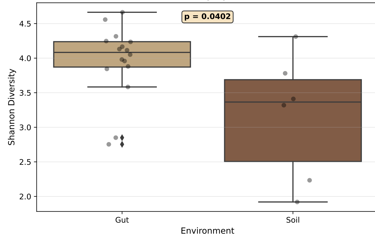
Shannon Diversity by Environment
