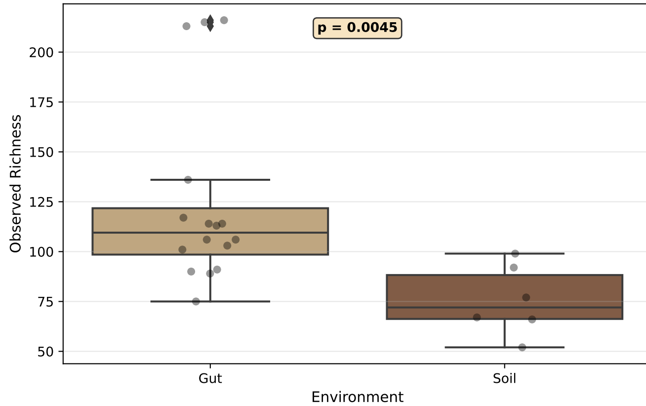
Observed Richness by Environment
