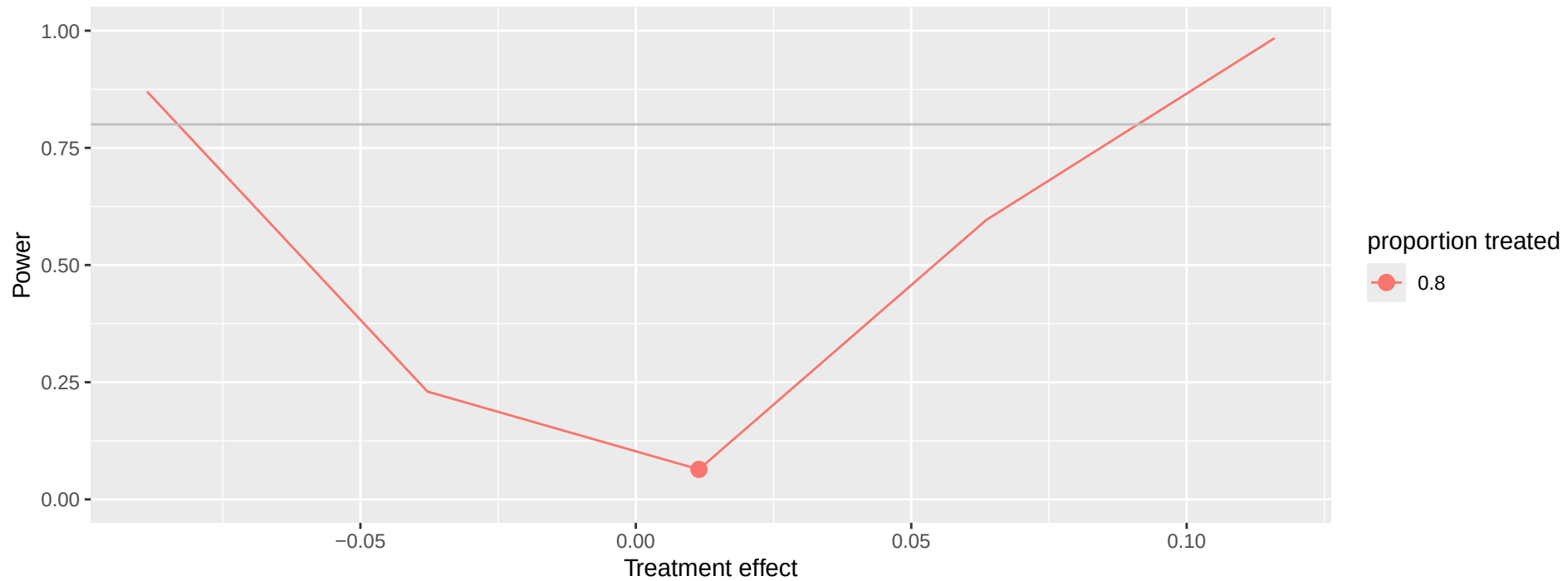
SalienceClim_any – scale from 0 to 1 n= 3500
