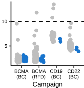
Average ipAE
