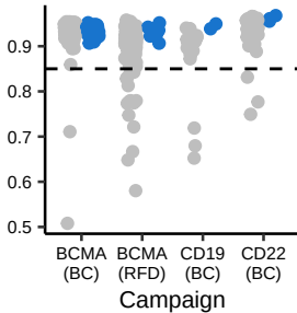
Average ipTM
