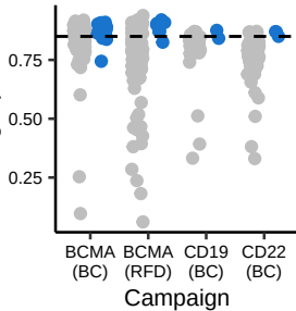
Average ipSAE
