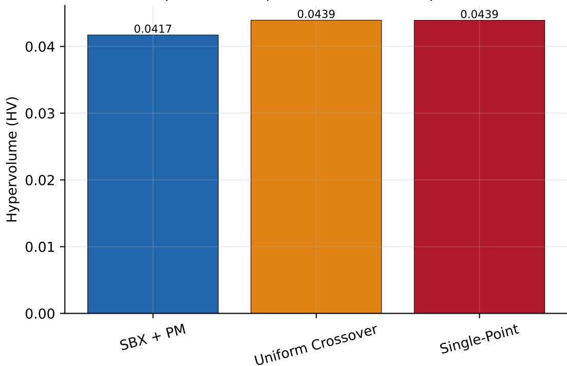
Search operator comparison (Decoder repair, NSGA-II)
