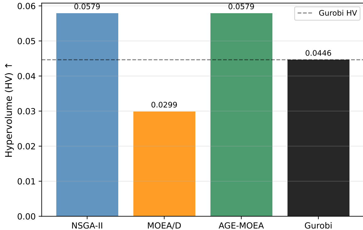
Final HV by Algorithm
