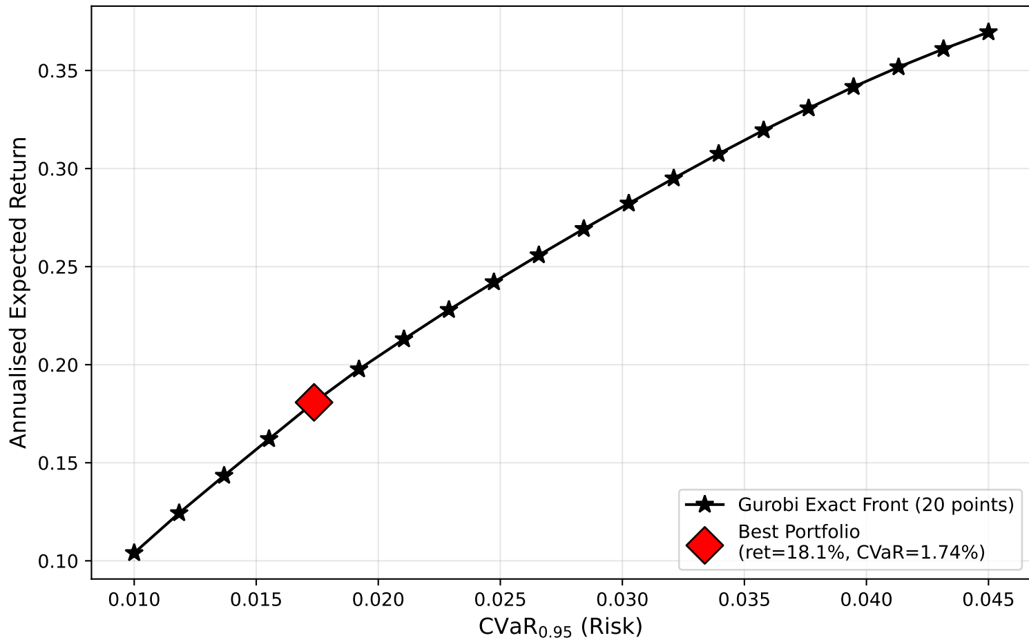
Gurobi Exact CVaR-Return Pareto Front (20-point \varepsilon -constraint sweep)
