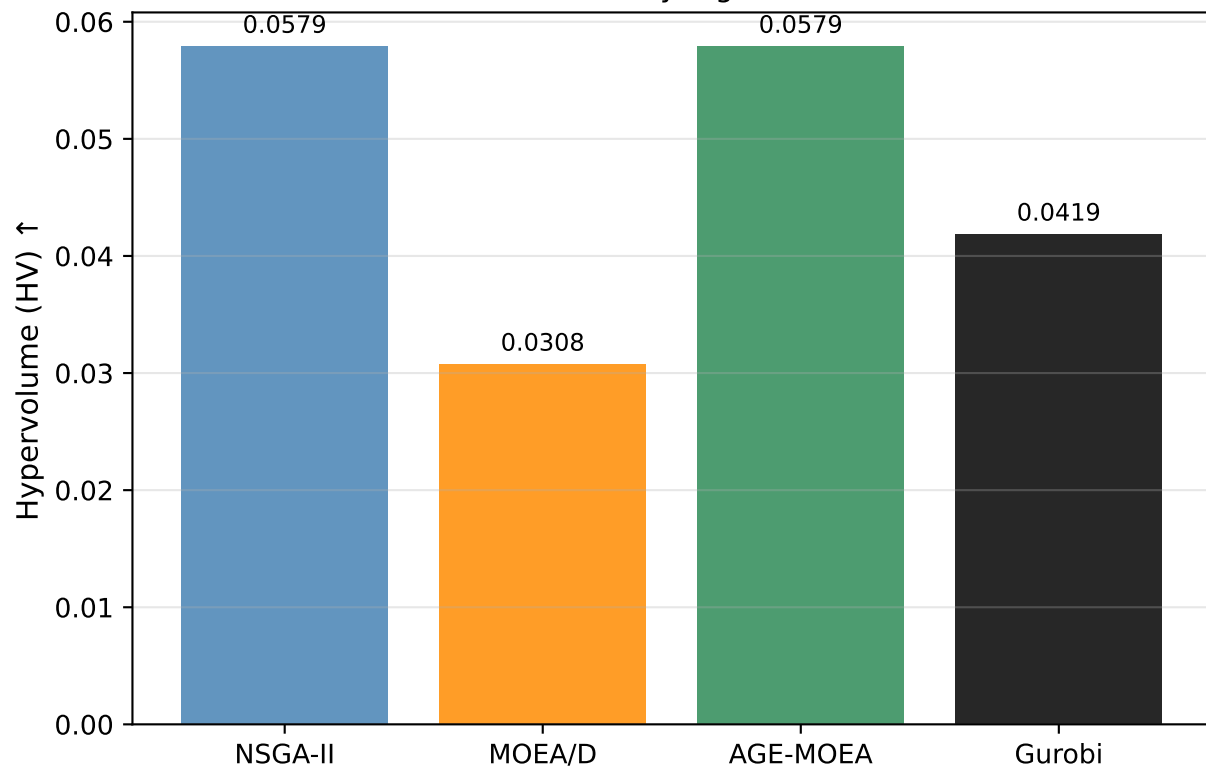
Final HV by Algorithm
