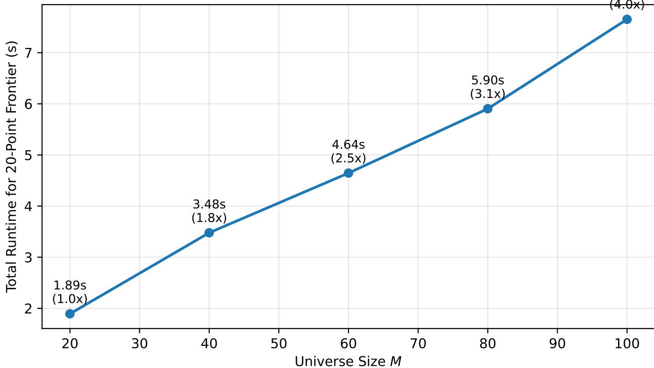
Stratified Gurobi \varepsilon -Constraint Scaling Full 20-Point CVaR Frontier per Universe Size
