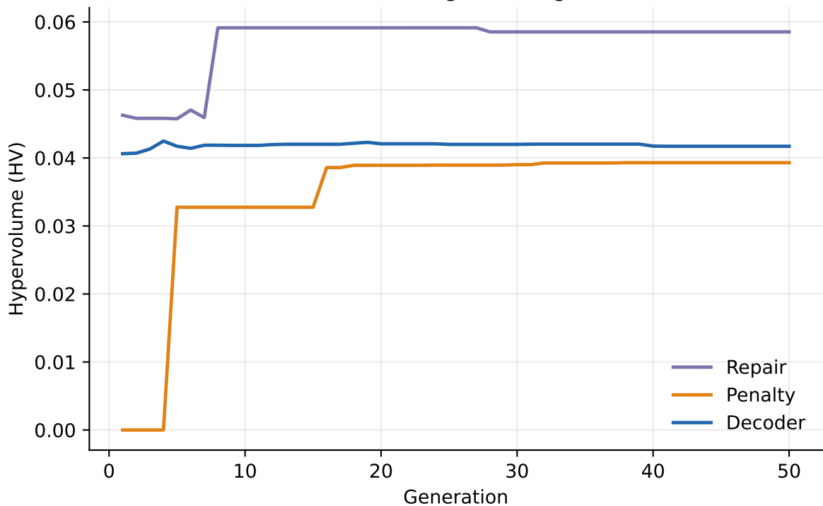
Constraint handling: HV vs. generation
