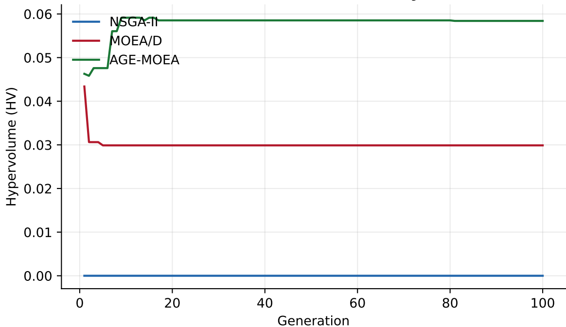
Convergence: HV vs. generation ( n_{gen} = 100 )
