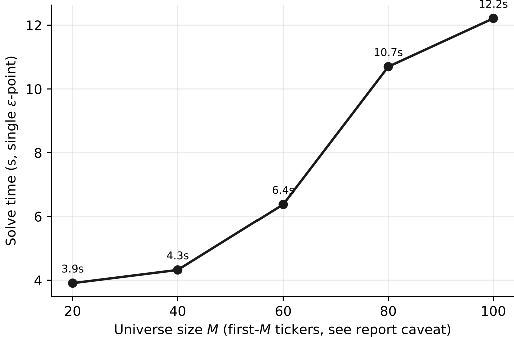
Gurobi exact MIQP runtime vs. universe size
