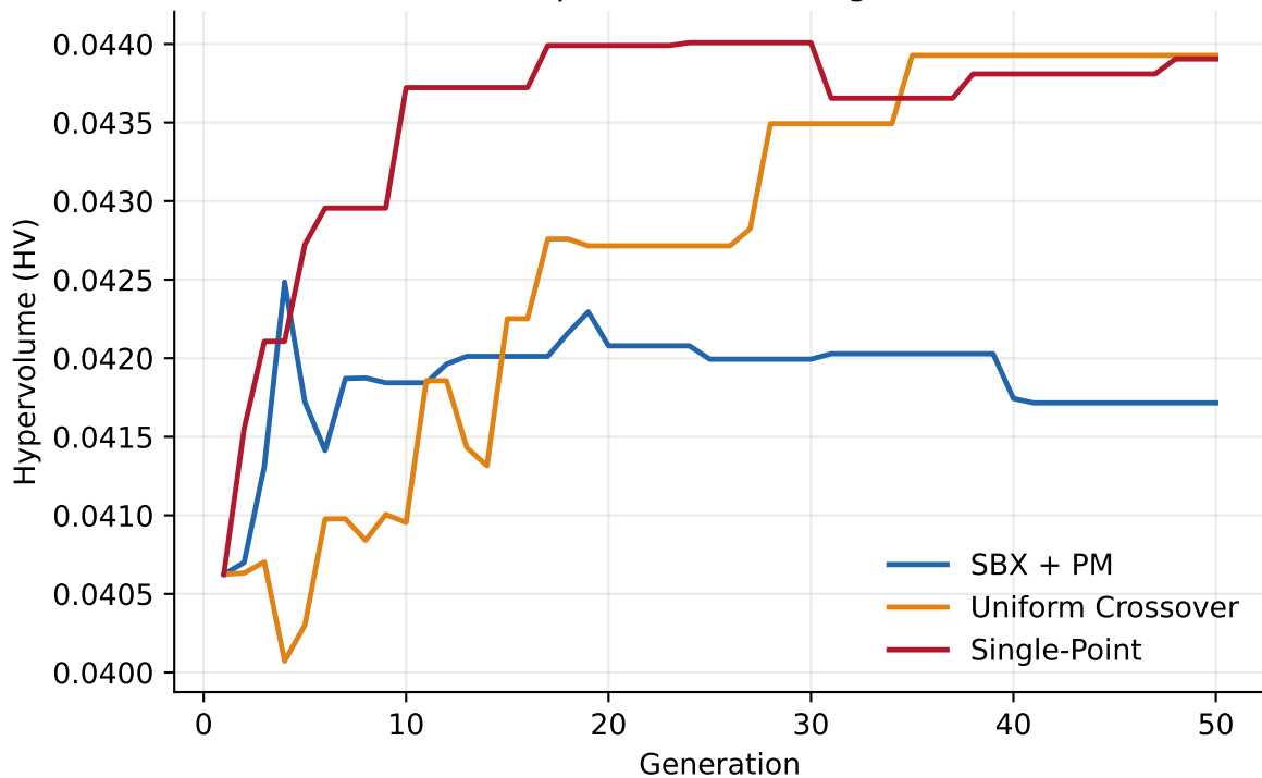
Search operators: HV vs. generation
