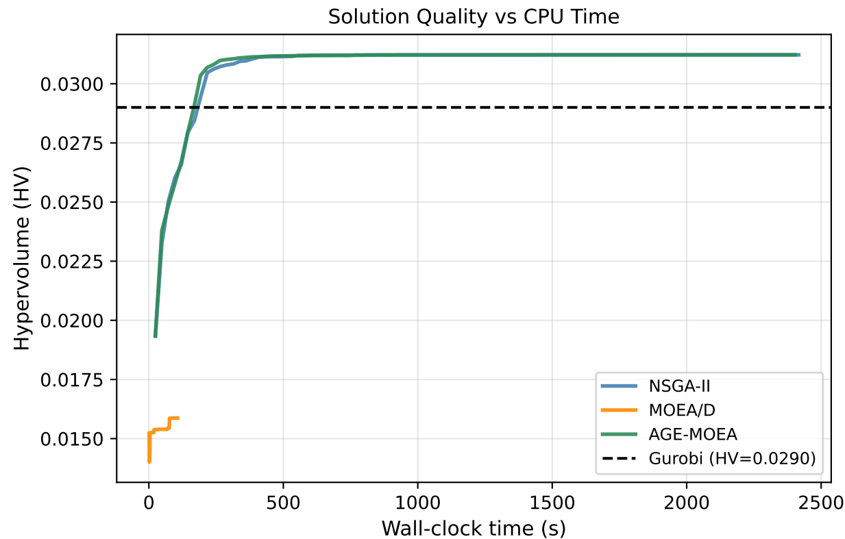
Algorithm Comparison: Solution Quality vs CPU Time & Iteration (pop=500, 100 generations, seed=42) Note: time axis is interpolated from available total runtime
