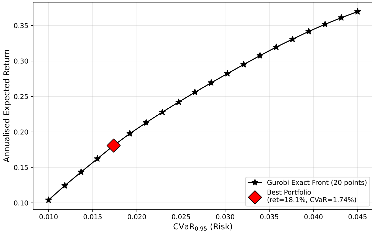
Gurobi Exact CVaR-Return Pareto Front (20-point \varepsilon -constraint sweep)
