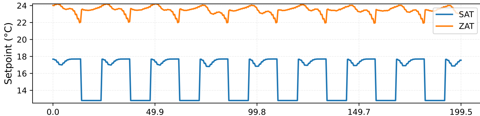
Control Inputs (SAT and ZAT)
