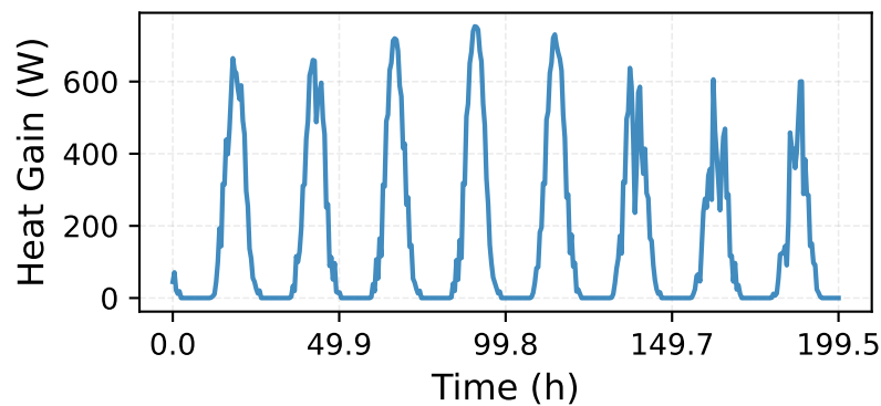
Solar Heat Gain
