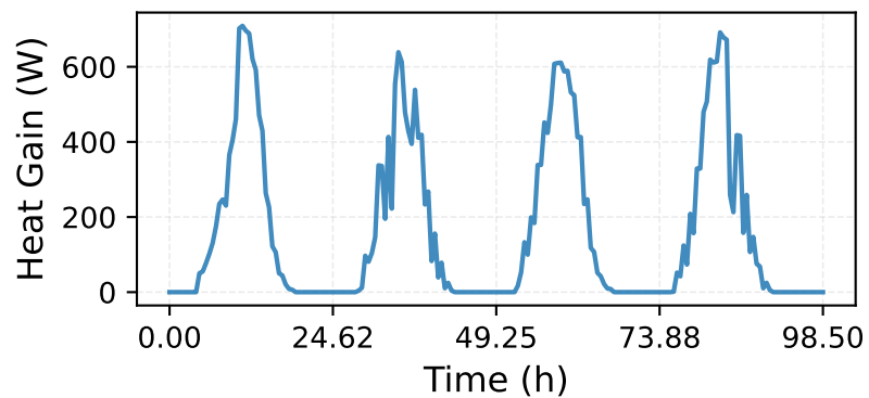
Solar Heat Gain
