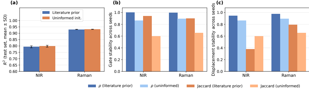
Figure 3: H4: literature-informed prior versus uninformed initialization, 10 training seeds. (a) Predictive performance does not differ beyond seed-to-seed variability. (b) Stability of the final gate across seeds is substantially higher with the literature-informed prior, in both modalities. (c) Stability of the learned displacement d = g_{\text{final}} - g_0 : the prior also stabilizes what the model learns, not only where it starts. In the uninformed condition g_0 is constant, so panels (b) and (c) coincide there by algebraic identity.
