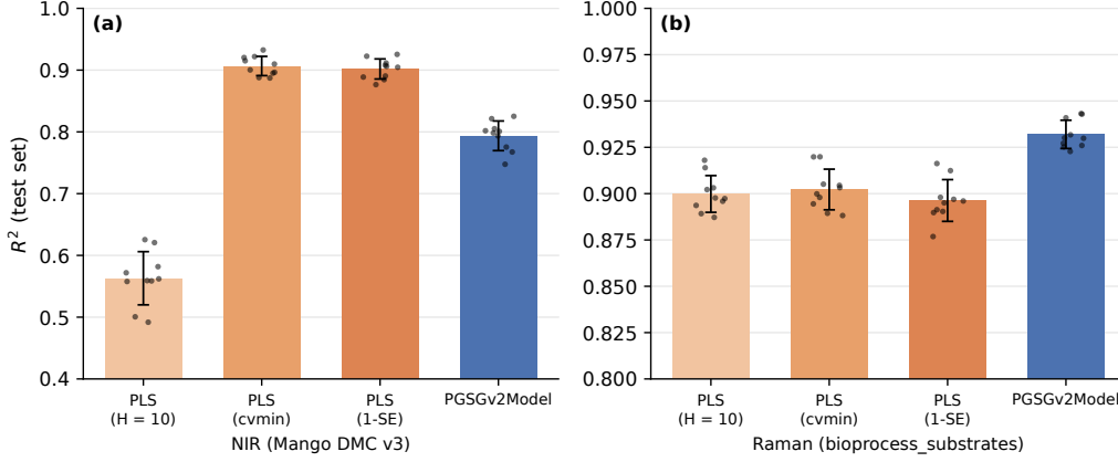
Figure 1: H1: test-set R^2 over ten paired splits, grouped by sample, for PLS with fixed H = 10 , PLS with cross-validated H (cvmin and one-standard-error rules), and PGSGv2Model. Bars: mean; error bars: SD; points: individual splits.
