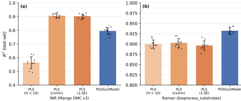
Figure 1: H1: test-set R^2 over ten paired splits, grouped by sample, for PLS with fixed H = 10 , PLS with cross-validated H (cvmin and one-standard-error rules), and PGSGv2Model . Bars: mean; error bars: SD; points: individual splits.
