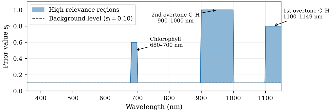
Literature-based prior \mathbf{s} for mango DMC% (NIR)
