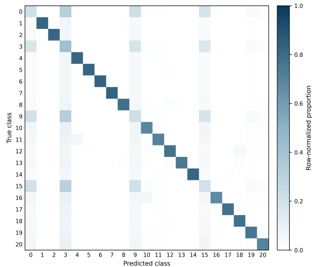
Figure 3: Row-normalized confusion matrix for the frozen XGBoost model on the official test partition.
